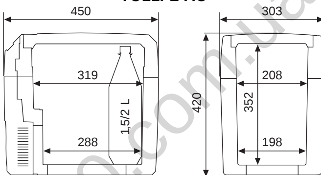
TC21FL-AC
