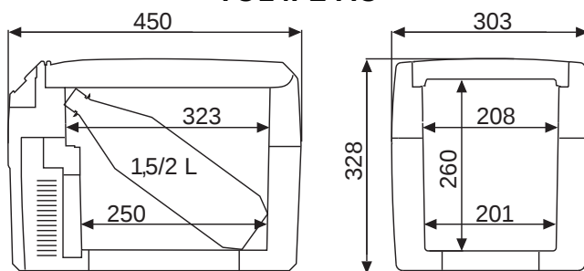
TC14FL-AC
