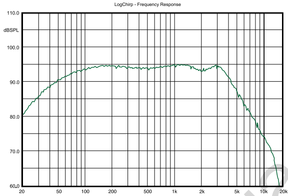
Tweeter HGC-2.28T (Fig.5.2)
