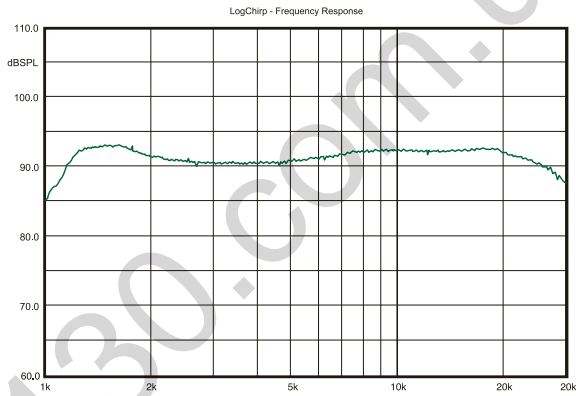
Crossover HDC-2.23C
