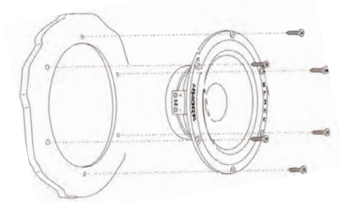
Installation of the midwoofer speaker together with grill
