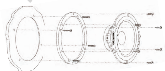
Installation of the midwoofer speaker with using of spacers
