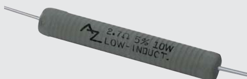
Resistori a bassa induttanza parassita Low inductance resistors
