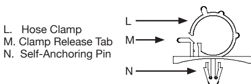
(Fig. 3) Leader Hose Bracket (N/A 32534)
