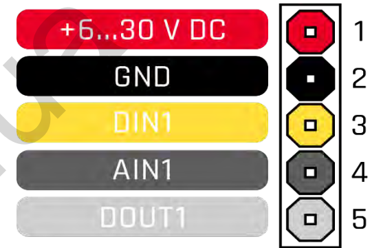
Figure 2 MTB100 pinout
