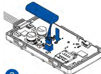
Figure 6 Battery connection
