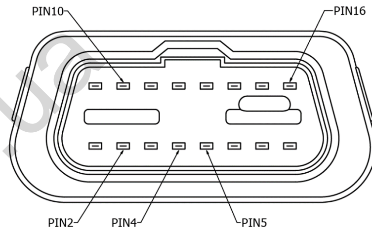
Figure 2 FMB020 OBDII socket pinout
