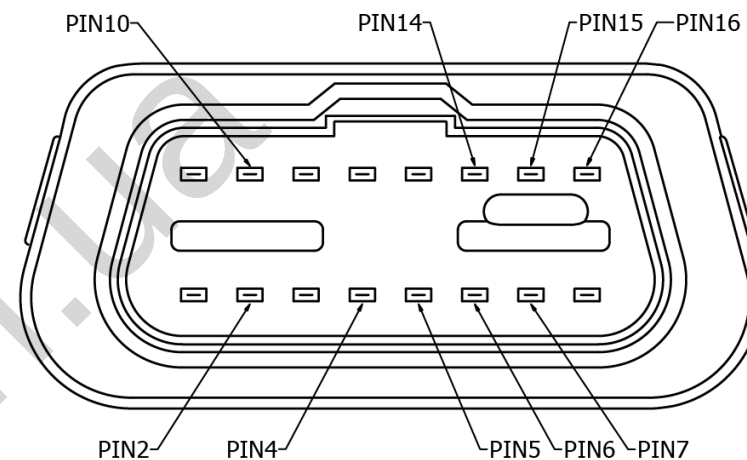
Figure 2 FMB003 OBDII socket pinout
