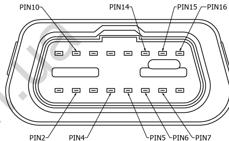
Figure 2 FMB002 OBDII socket pinout
