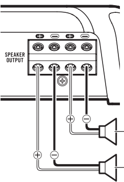
Speaker output
