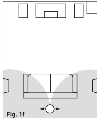
Fig. 1f 7.1 Rear Placement using One H65-SM Speaker
