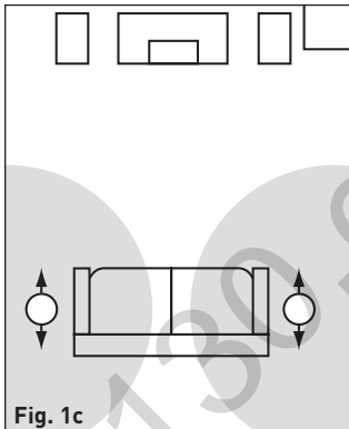
Fig. 1c 5.1 Surround Placement using Two H65-SM Speakers
