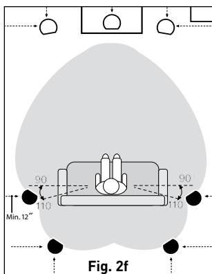
Direct-Radiating Speakers in a 7.1 placement
