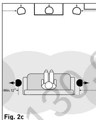
5.1 Surround Placement, diffuse soundfield
