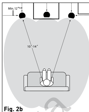
Front Left, Center, Right Speakers
