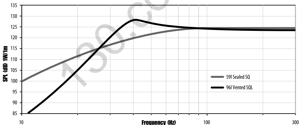
Frequency Response
