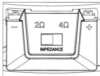
2-Ohm Setting
