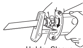
Holder Sleeve
