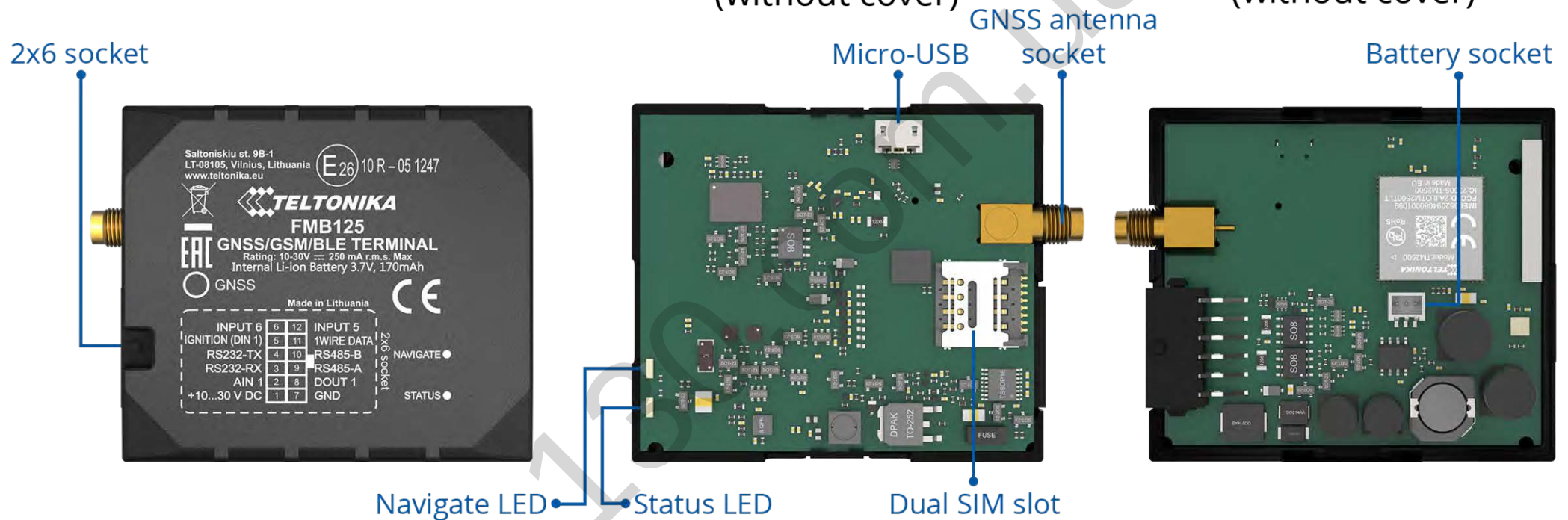
Top view (without cover)
