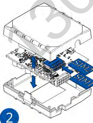
Figure 5 SIM card insert
