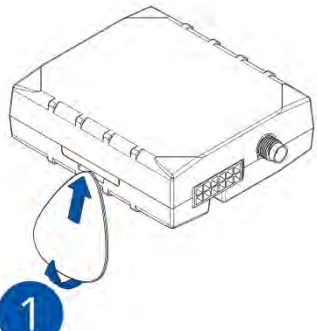
Figure 4 Cover removal
