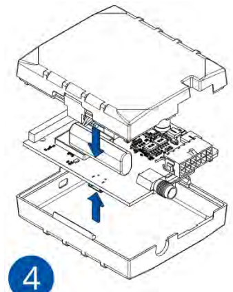
Figure 7 Attaching cover back
