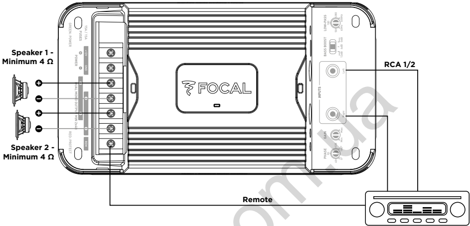
fig. 3.3 ter - FDS 1.350, speaker pair wiring
