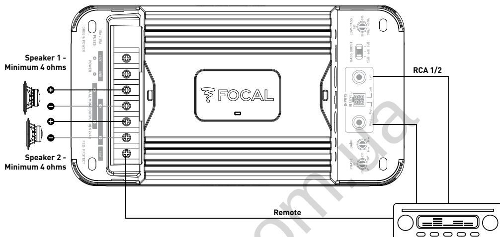
fig. 3.3 ter - FD 1.350, speaker pair wiring
