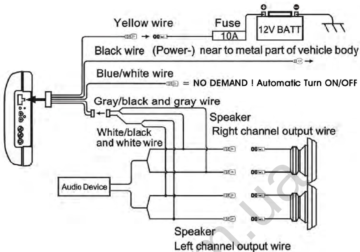
Wiring Diagram1 (High level input)
