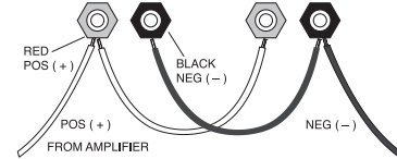
Figure 1. Parallel connection
