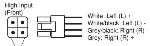
Hi level input plug on amp
