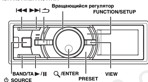
iDA-X311/iDA-X311RR
