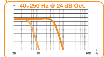
LO-PASS FILTER
