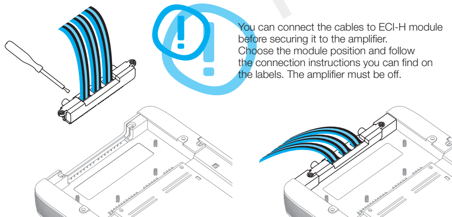
■ Flush mounting
